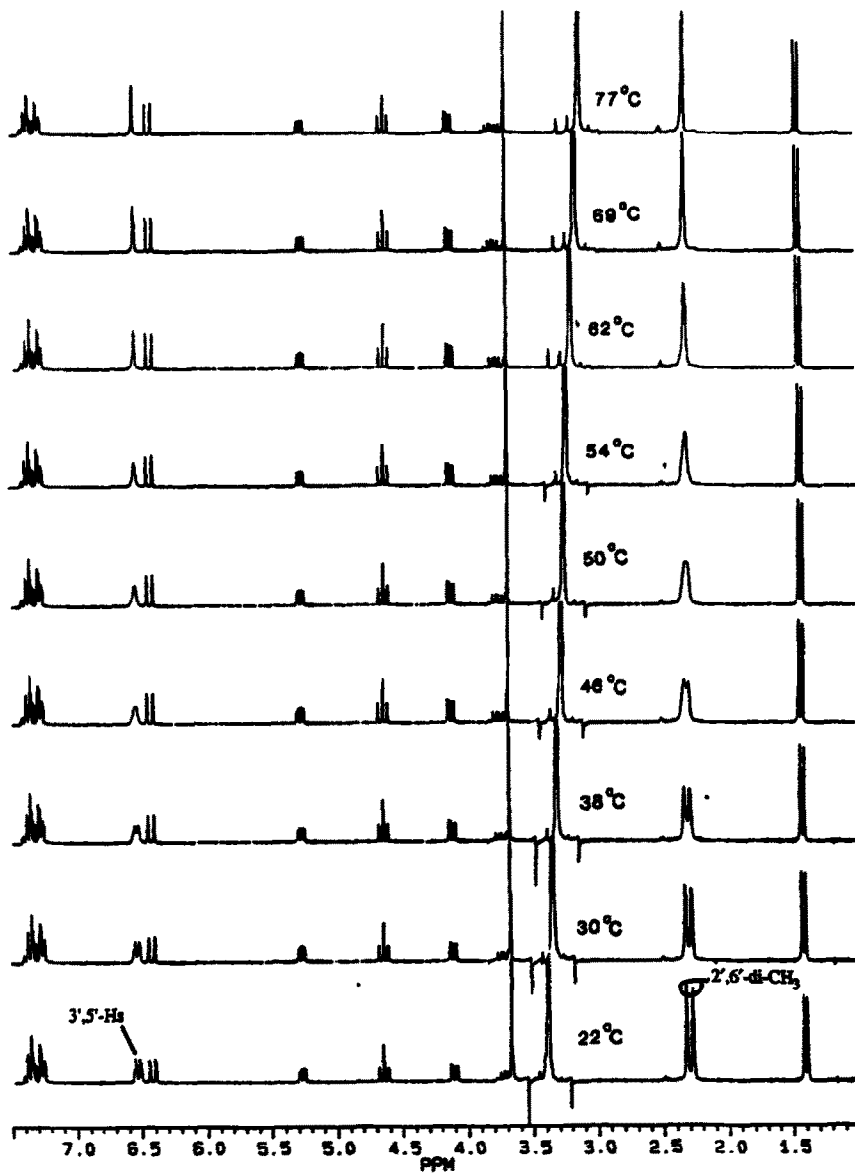
Figure 1. Proton NMR spectra of compound 1 in DMSO- d_6 at different temperatures, showing the coalescence (at 30°C) of the two aromatic methyl resonances at \sim 2.3 ppm.
